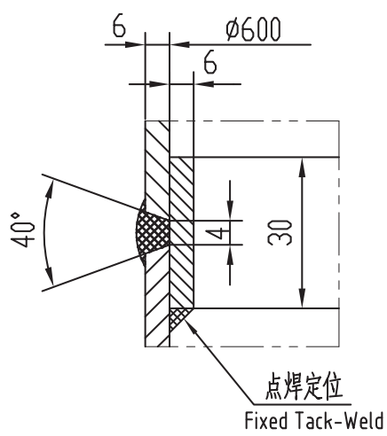
B1,B2 焊接详图 Welding detail of B1,B2 NO SCALE
