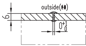
A1 焊接详图 Welding detail of A1 NO SCALE
