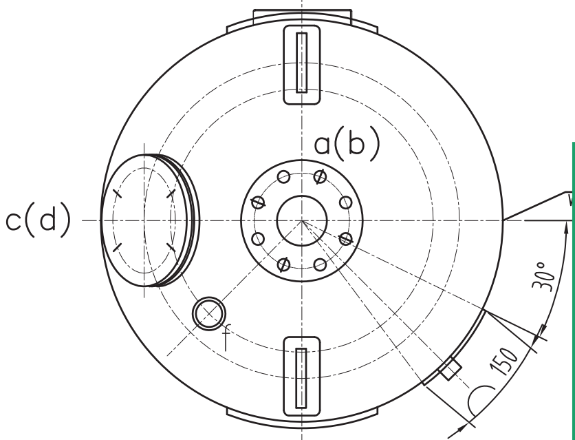
左吸附器方位图 Left adsorption cartridges diagram
