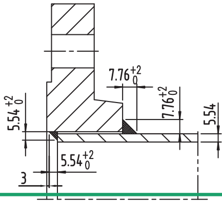
C3,C4 焊接详图 Welding detail of C3,C4 NO SCALE
